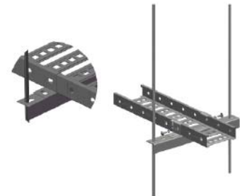
BC3-HDU Hold Down Unit
