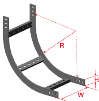
BL2-IR Inside Riser
