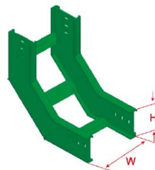
BL7-IR Inside Riser
