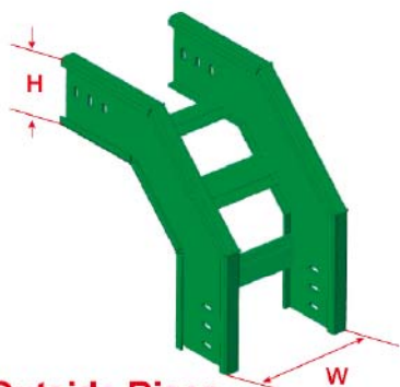
BL7-OR Outside Riser
