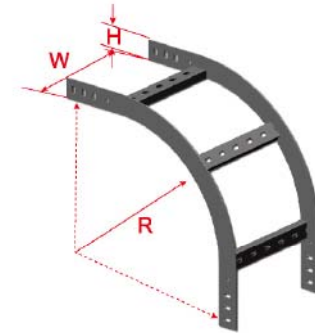
BL2-OR Outside Riser
