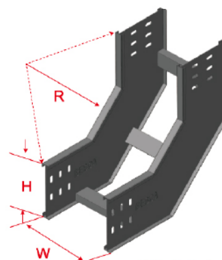
BL4-IR Inside Riser
