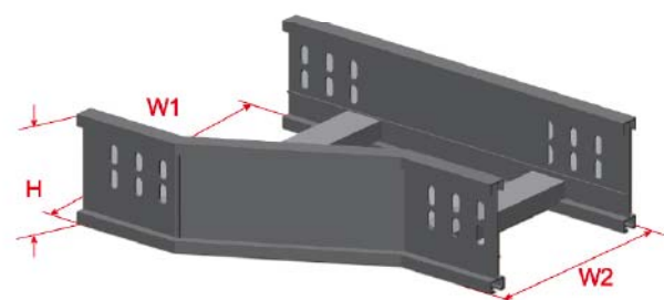
BL4-RR Right Hand Reducer
