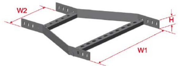
BL2-MR Middle Reducer
