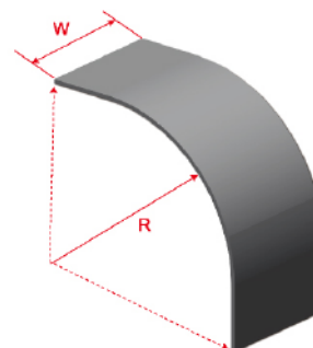
BL-ORC Outside Riser Cover
