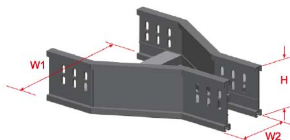
BL4-MR Middle Reducer
