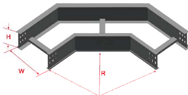
BL4-E Elbow 90°
