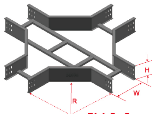
BL4-C Cross
