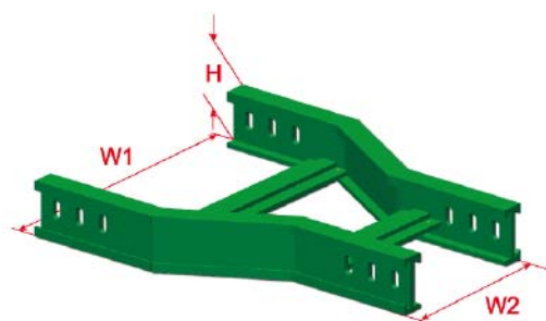
BL7-MR Middle Reducer
