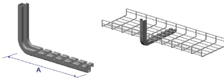
BM-LB L Bracket
