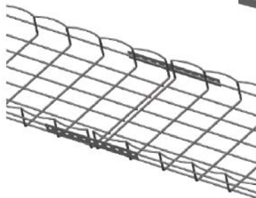
BM-SBL Splice Bar (Long)
