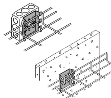
BM-WB Wall Bracket
