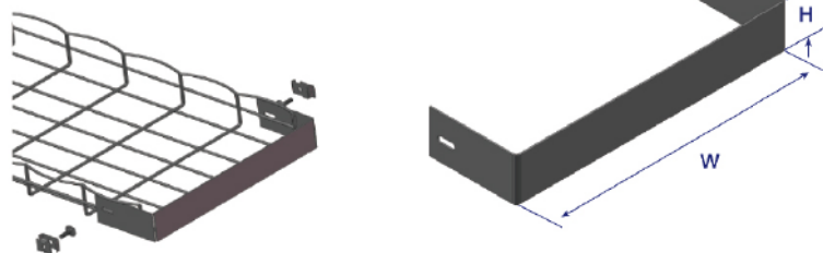
BM*-BE Blind End
