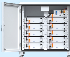
BOS-G50 Pro +BOS-G55-Cabinet (IP55) 51.2 kWh
