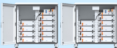
BOS-G45 Pro*2 + BOS-G55-Cabinet(IP55)*2 92.16 kWh
